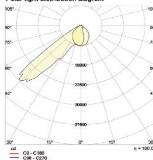
Polar light distribution diagram
