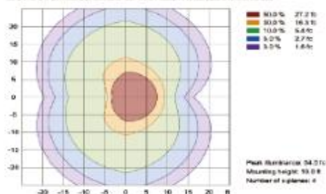
ISOFOOTCANDLE LINES OF HORIZONTAL ILLUMINANCE
