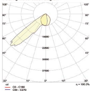
Polar light distribution diagram
